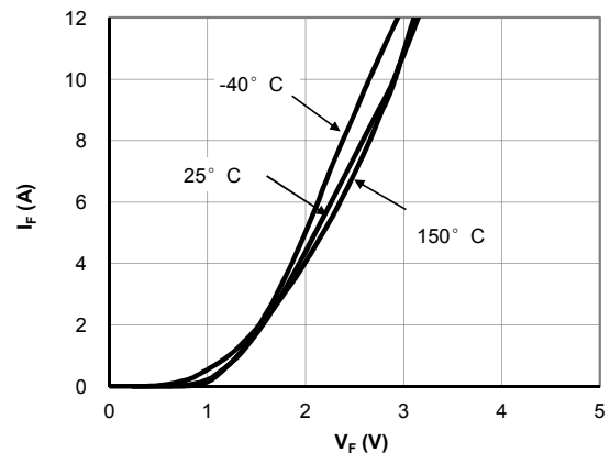
Figure 4: Diode Characteristic
