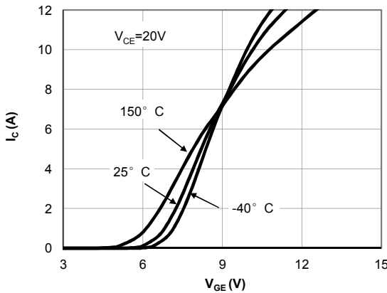
Figure 3: Transfer Characteristic
